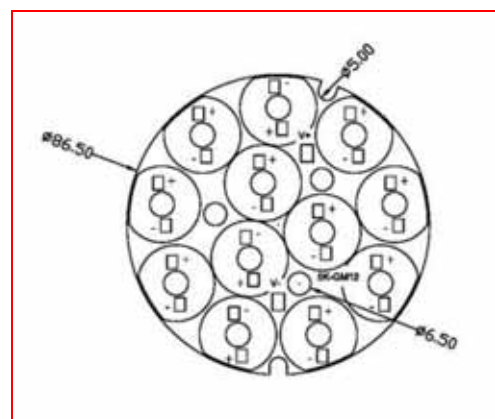
2. LED Module. (φ =86.5mm)
